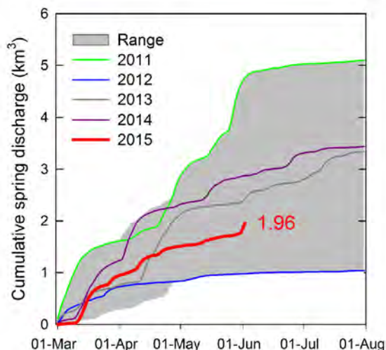
Figure 2. Cumulative discharge starting March, compared to the range from 2000-2014 (gray and the most recent past years). The red line and text denotes data through June 2. Because of the storm on May 31, we are using discharge to show the magnitude of the event. The phosphorus load typically follows discharge, and the nutrient loads also remain below those of 2014 at this time. The phosphorus load for this event will be reported next week.
